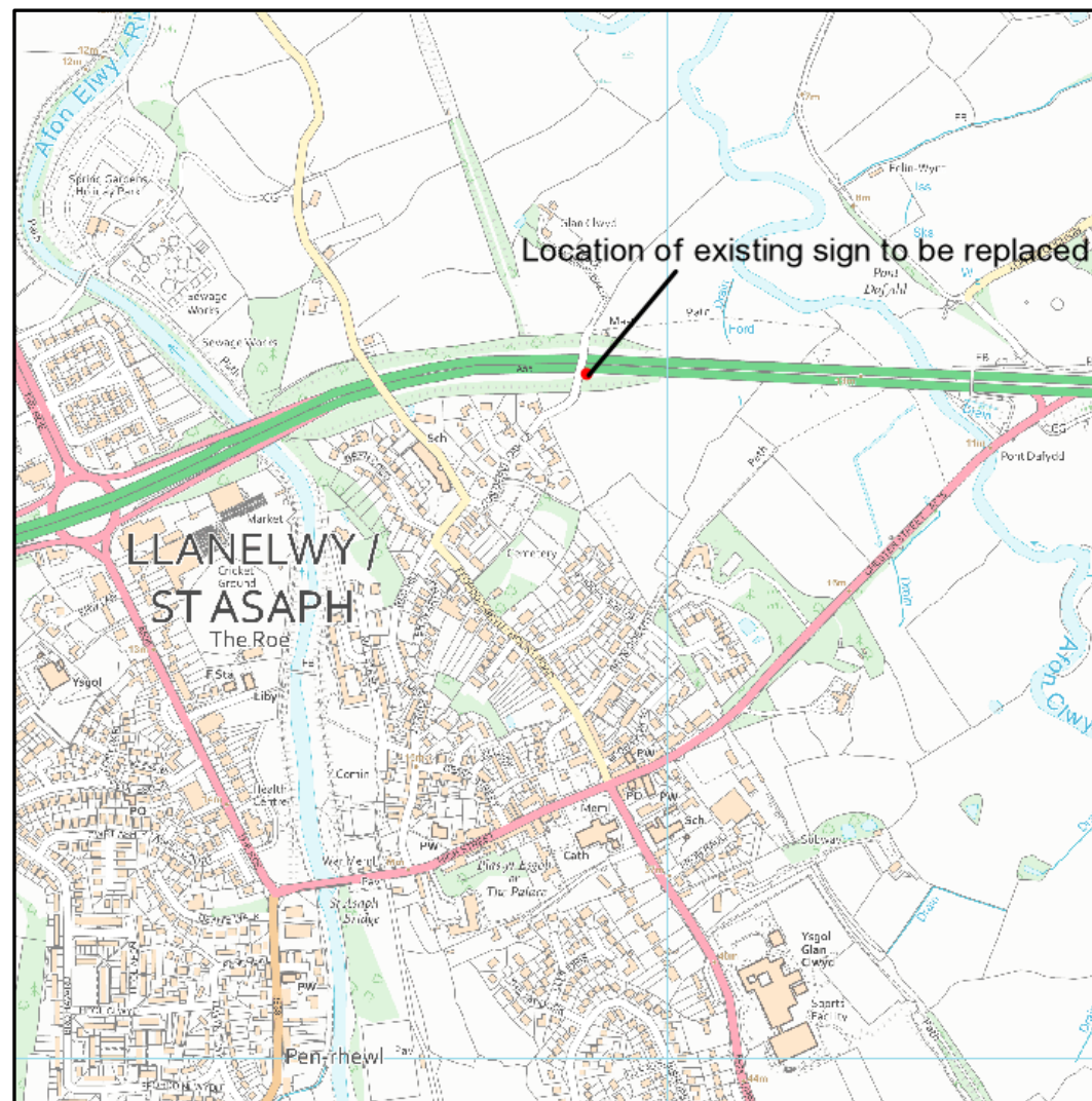
Location of existing Rhyl A55 brown sign on westbound carriageway in advance of Junction 27 (Talardy)
